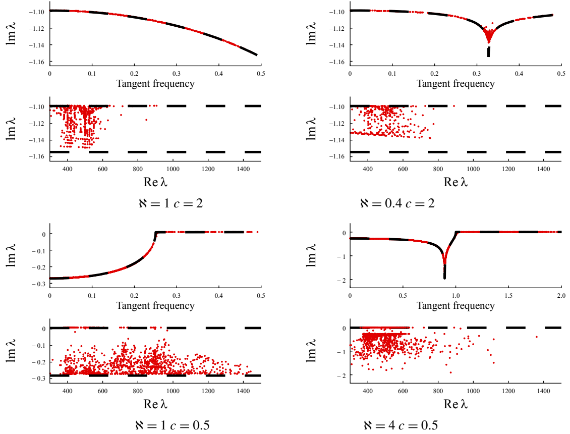
Figure 10. Numerically computed resonances for the transparent obstacle problem with various c and \mathfrak{N} when \Omega = B(0, 1) \subset \mathbb{R}^2 . In this case, we expand the solutions to (3) as u_i(r, \theta) = \sum_n u_{i,n}(r)e^{in\theta} and solve for some of the resonances with \text{Re } \lambda \sim 800 . In the lower graphs of each of the four subfigures, the red circles show \text{Im } \lambda vs. \text{Re } \lambda . The dashed black lines show the upper and lower bounds for \text{Im } \lambda when \mathfrak{N} corresponds to TE waves and the upper bounds on \text{Im } \lambda when \mathfrak{N} corresponds to TM waves from Theorem 1.2. Notice that by orthogonality of e^{in\theta} and e^{im\theta} for m \neq n , the pair (u_{1,n}e^{in\theta}, u_{2,n}e^{in\theta}) satisfies (3). In the top graph of each subfigure, the red circles show \text{Im } \lambda vs. n/\text{Re } \lambda for such pairs. That is, we plot \text{Im } \lambda vs. the scaled tangent frequency of the resonance state. The dashed curve shows a plot of (cr_1/(2l_1))(c\xi) , the decay rate predicted for a billiards trajectory traveling with scaled tangent frequency c\xi . The large spikes in the top graphs occur at the Brewster angle when \mathfrak{N} corresponds to TM waves.
