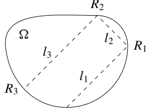
Figure 1. Path of a wave packet along with the lengths between each intersection ( l_i ) and the reflection coefficient at each point of intersection with the boundary ( R_i ). After each reflection with the boundary, the amplitude of the wave packet inside \Omega decays by a factor of R_i . If the speed of the wave is c , the time between reflections is given by c^{-1}l_i .
