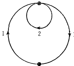
FIGURE 2. A quotient graph with one vertex and two edges, imbedded in the projective plane, with voltages in Z_4 , leading to a minimal imbedding of the complete graph K_4 in the sphere T_6 .
