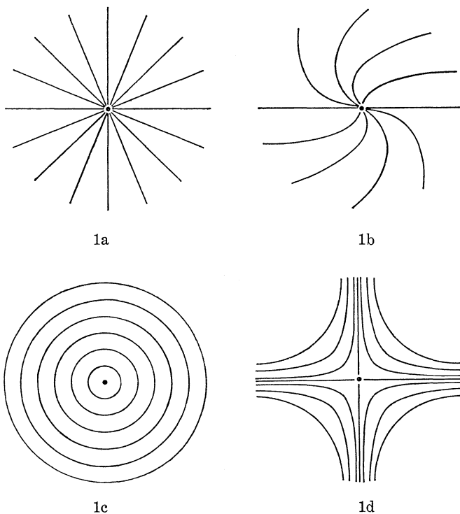
FIGURE 1. Orbit structures of R acting on R^2 for various semidirect products.
