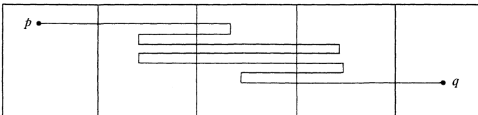
FIGURE 1 Only the nerve of C_1 in C_0 is shown.
