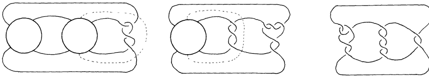
Typical elementary tangles
