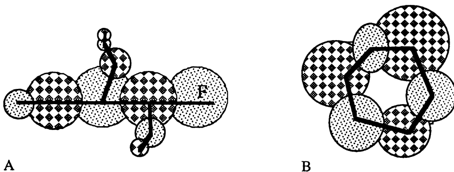
FIGURE 2.4.1. Since the exterior is assumed to be connected as in A , the associated graph has an endpoint in a component with two edges and two vertices. If the exterior were disconnected, then a cycle as in B could result.
