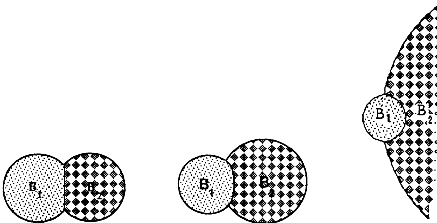
FIGURE 2.3.2. As \theta varies, a unique standard double bubble represents every possible ratio of \text{area}(B_1) to \text{area}(B_2) .
