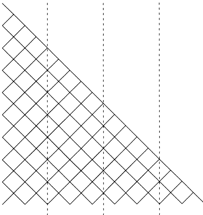
FIGURE 1.1. Critical lines
