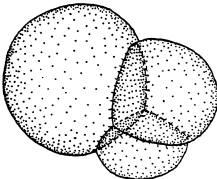
FIGURE 1.1.2. It is an open question whether the standard triple bubble is the least-area way to enclose three given volumes. (Jim Brecht) [M10].
