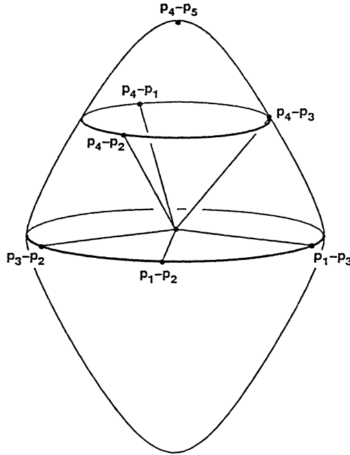
FIGURE 3.4.3. The unit \Psi_2 -ball. All five vertices of the regular tetrahedron and its reflection are unit \Psi_2 -distance apart.
