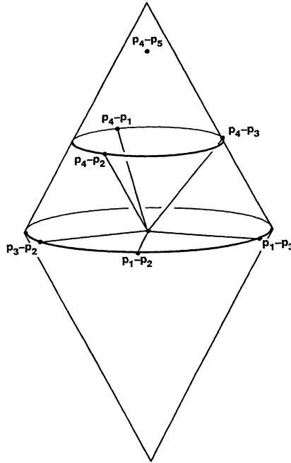
FIGURE 3.4.2. The unit \Psi_0 -ball. All six sides of the regular tetrahedron have \Psi_0 length 1 as well.
