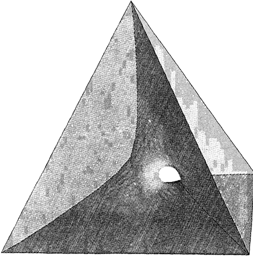
FIGURE 1.1.1. It is an open question whether the tetrahedron bounds a smaller soap film which does not separate the four regions. This figure was done by Jean Taylor of Rutgers University and The Geometry Center, following an idea due to Bob Hardt.
