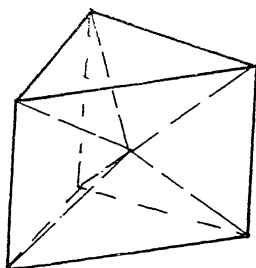
FIGURE 3.5.1. The cone over the triangular prism is \Phi -minimizing.
