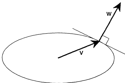
FIGURE 3.1.1. The vector w is dual to v .
