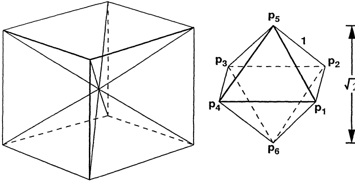
FIGURE 2.2.1. The cone over the cube is energy-minimizing if interfaces between opposite regions are \sqrt{2} times as costly as between adjacent regions. The proof uses the dual polyhedron, the unit regular octahedron, where opposite points are a distance \sqrt{2} apart.
