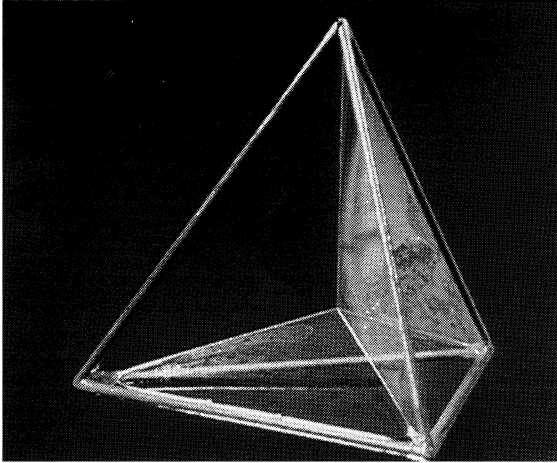
FIGURE 1.0.1. The cone over the tetrahedron provides the least-area soap film which separates the four regions.
