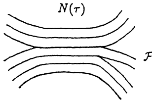
an example of \mathcal{F} (represented as a partial foliation) and \tau not suited to \mathcal{F}
