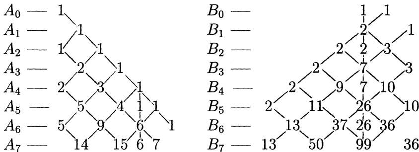
FIGURE 1. The Bratteli diagrams of (A_n) and (B_n) .
