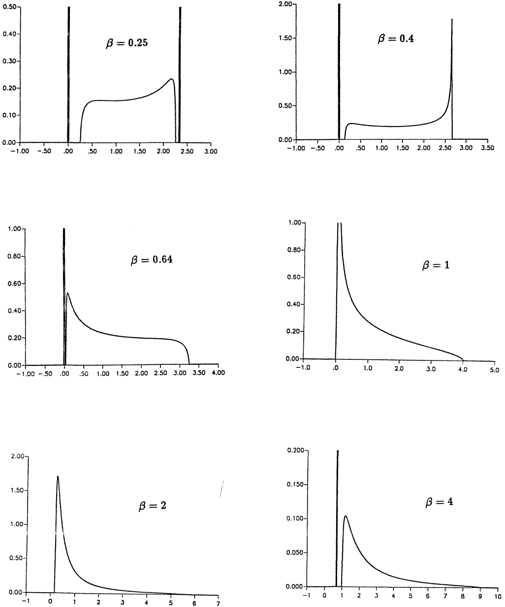
Figure 2. c-free Poisson distribution \pi_{\alpha,\beta} for fixed \alpha = 1 and six different values of \beta ; vertical double lines indicate \delta -peaks; note that the \delta -peak at z_0 lies first on the right side of the continuous spectrum, then it disappears and reappears again on the left side of the continuous spectrum.
