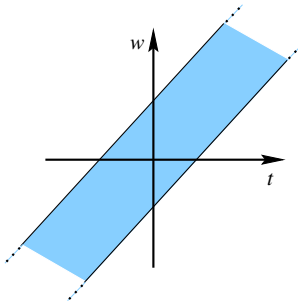
Figure 2.3. The Thurston norm ball of M_\gamma .
