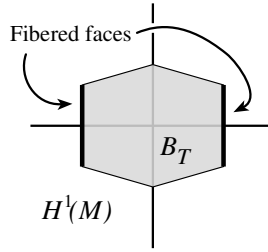
Figure 1.3. The Thurston norm ball.
