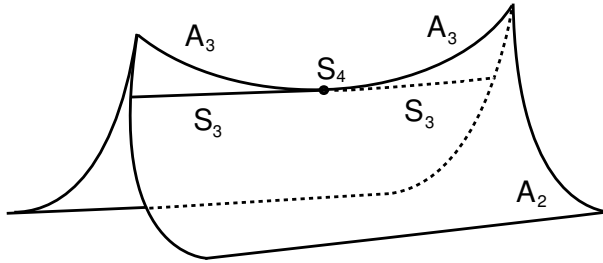
Figure 1. S_4 -caustic.
