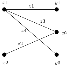
Figure 2. The underlying graph in Figure 1.
