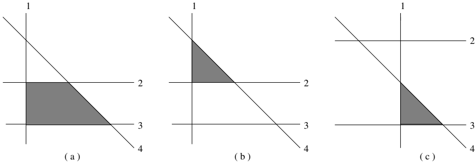
Figure 2. Three arrangements related by flipping coorientations and translating hyperplanes.
