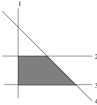
Figure 1. A hypertoric variety of real dimension 8 obtained by reducing \mathbb{H}^4 by T^2 .
