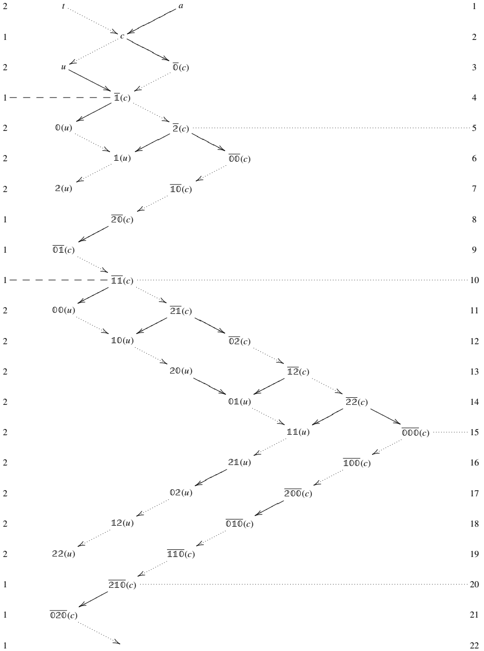
Figure 4. The beginning of the Lie graph of \mathcal{L}(\Gamma) . The generator ad(t) is shown by plain arrows, and the generator ad(a) is shown by dotted arrows. The left row indicates the dimensions of \mathcal{L}_n .
