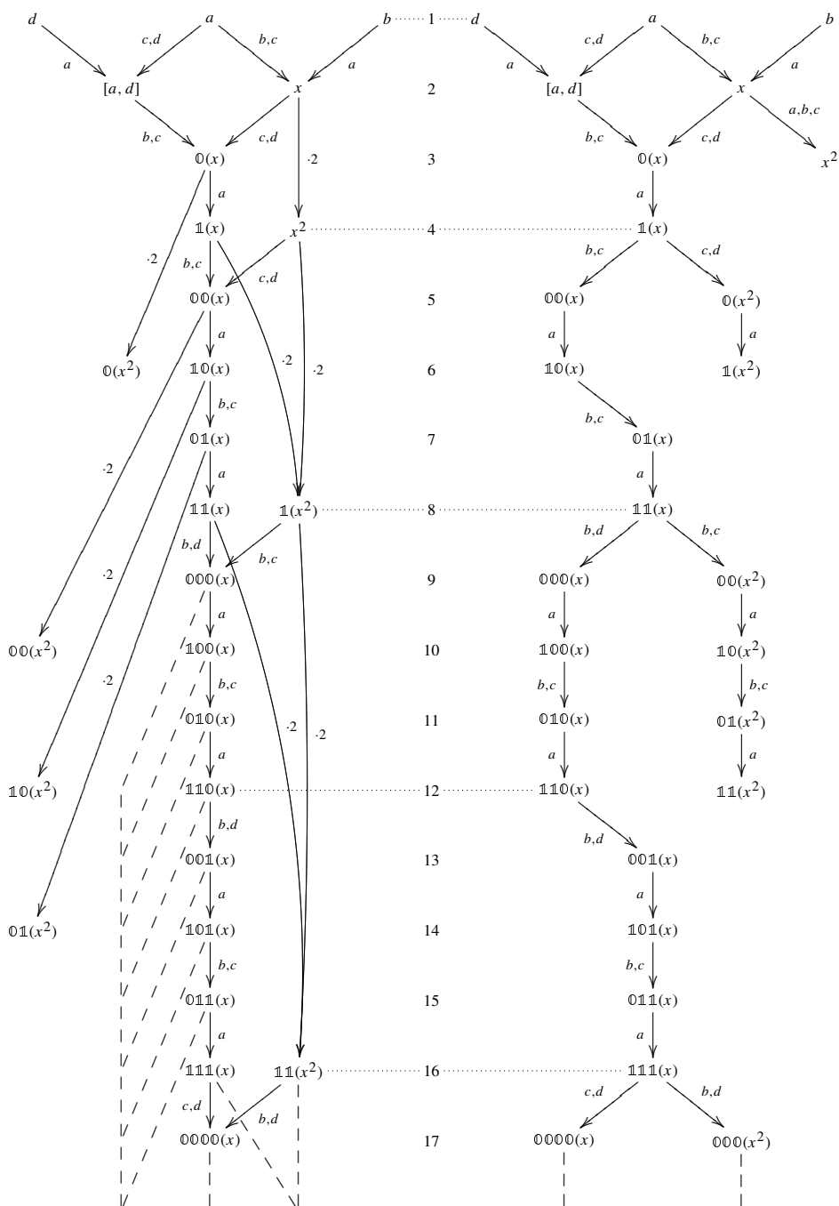
Figure 2. The beginning of the Lie graphs of L_{\mathbb{F}_2}(\mathcal{G}) (left) and L(\mathcal{G}) (right).
