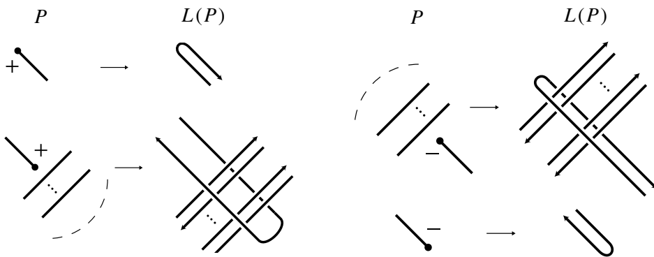
Figure 11. l(P, x, \epsilon_x) .
