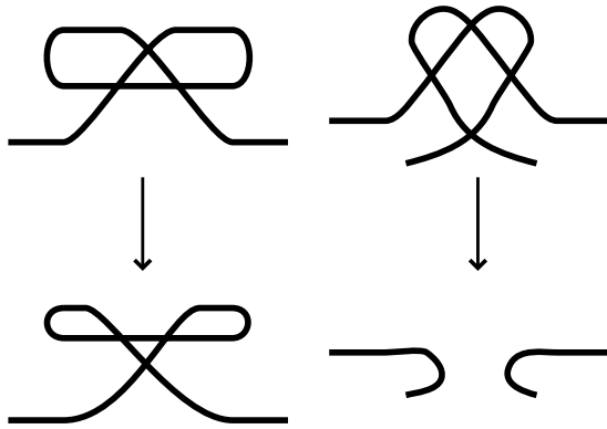
Figure 10. Transformations on certain (almost) ordered Morse divides.
