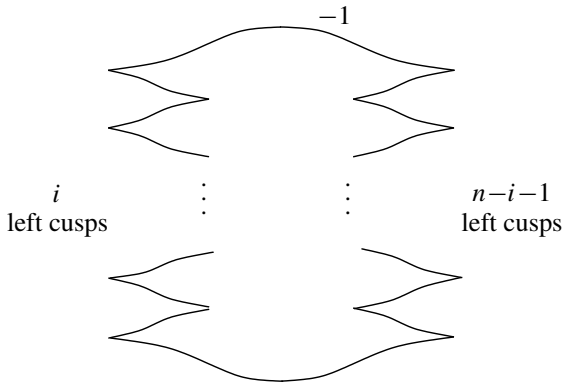
Figure 10. The contact structure \eta_i on L(n, 1) .
