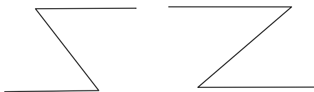
Figure 3. The two possible “zig-zags”.
