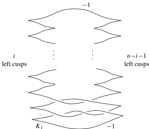
Figure 9. Contact structures on the three-manifold -\Sigma(2, 3, 6n-1) .
