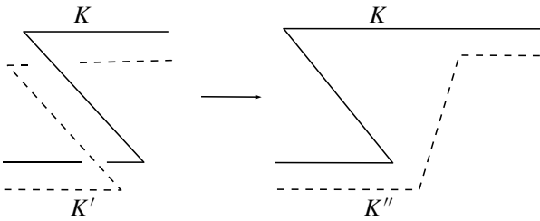
Figure 4. Modification of the Legendrian push-off.
