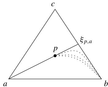
The Hilbert geometry of a 2-simplex is not uniquely geodesic.
