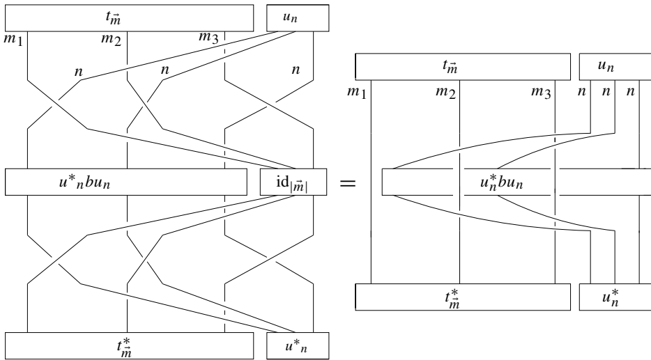
Figure 11. Pictorial representation of \text{Shift}_m^M(b) \in A_{|\vec{m}|+sn} , for b \in A_{sn} ( s=3 ).
