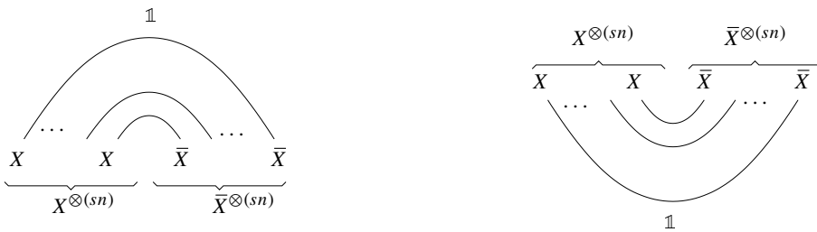
Figure 16. \iota_{X^{\otimes(sn)}}^* and \iota_{X^{\otimes(sn)}} .
