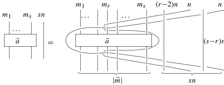
Figure 15. (\tilde{a} \otimes 1_{sn}) = x_r(\tilde{a} \otimes 1_{sn})x_r^* .
