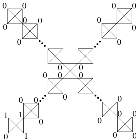
Figure 4. A function v defined on the first step graph of \mathcal{V}^L_n .
