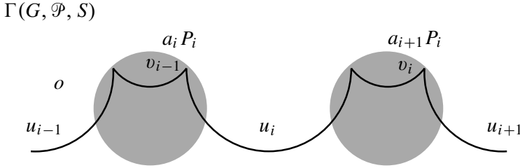
Figure 1. Part of the polygonal path o in \Gamma(G, \mathcal{P}, S) . For each i , the P_i -component of o containing the subsegment v_j is long with respect to the S -metric. This implies that the path o is a quasi-geodesic with different endpoints.
