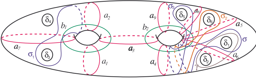
Figure 9. \Sigma_{2,6} .
