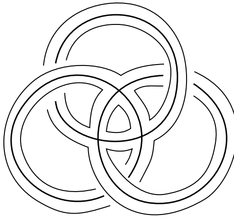
Figure 13. Natural “thickening” of the \text{III}^8 -type singular fiber.
