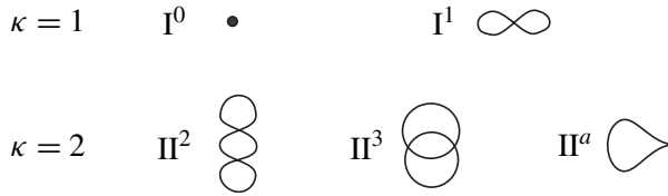
Figure 4. List of C^\infty equivalence classes of singular fibers of C^\infty stable maps of orientable 3-manifolds into surfaces.
