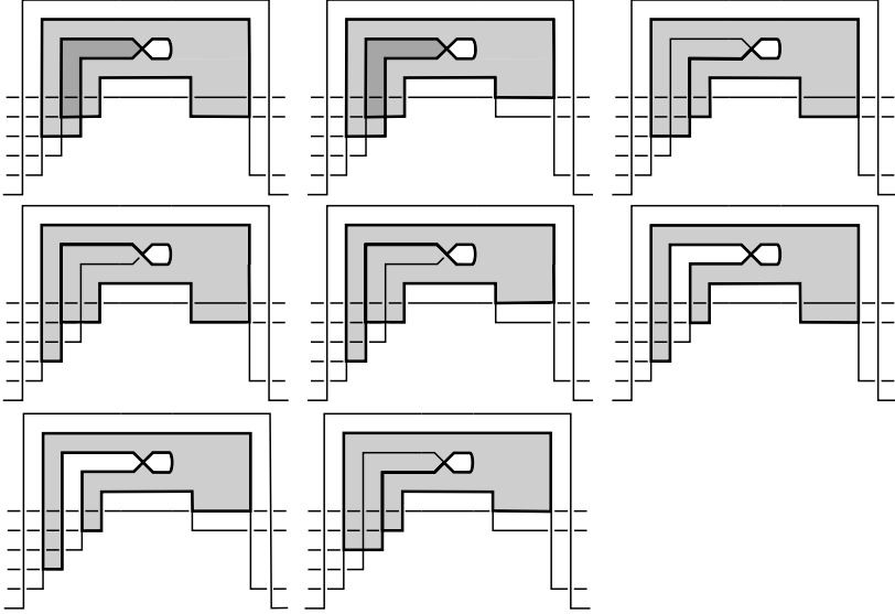
Figure 18. Disks contributing to L(\partial B_j) when I_j is of type (3). The boundary of each disk is highlighted.
