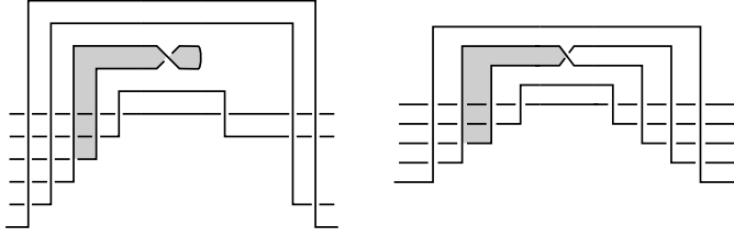
Figure 14. Disks contributing to \partial z_r and \partial q_s .
