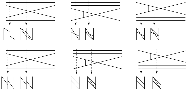
Figure 28. Sweeping V past a crossing with a handleslide immediately to the left. The top row will be switches and the bottom will be marked returns. In each row, we label the cases (1), (2) and (3) from left to right.
