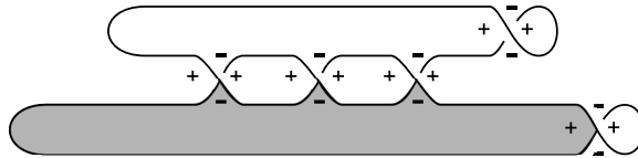
Figure 4. A convex immersed polygon contributing q_3q_2q_1 to q_5 . Crossings are labeled from left to right.
