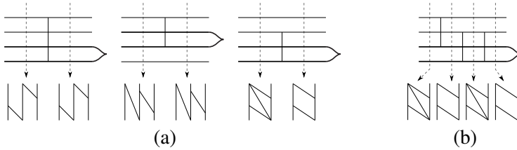
Figure 30. Left: the 3 possible local neighborhoods of the handlelide h_1 . Right: MCS move 17 at a right cusp introducing two new handleslides. The two dark lines correspond to the strands entering the right cusp.
