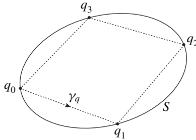
Figure 1. Closed curve \gamma_q and corresponding sequence of bounce points \mathbf{q} = (q_0, \dots, q_3) .
