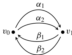
Figure 1. Ext quiver of the basic algebra B of the block \mathfrak{b}^{2,r}(\bar{\lambda}) of \tilde{u}_k(2, l) .
