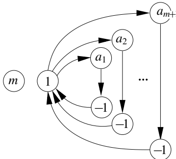
Figure 9. Reduction from coSUBSET SUM to ESSENTIAL.
