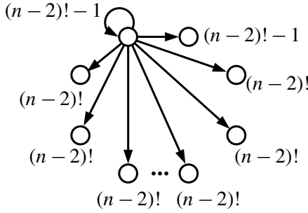
Figure 4. Vector in \mathbb{R}^{n^2} ; the vertices \{1, \dots, n\} are arranged clockwise. The number attached to a vertex gives the value on the edge going into this vertex.
