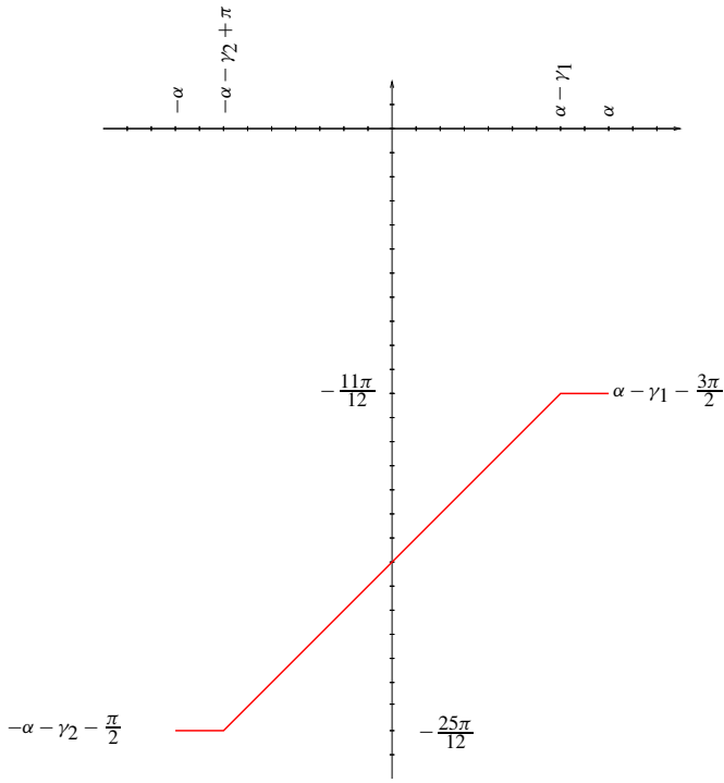
Figure 5. \{(\beta, \arg(\bar{m}_f(\beta)))\} at a D_2^+ corner; \alpha = \frac{3\pi}{4} , \gamma_1 = \frac{\pi}{6} , \gamma_2 = \frac{5\pi}{6} .
