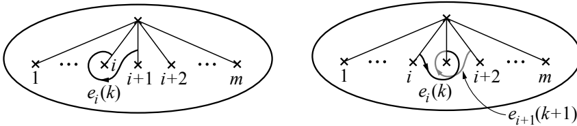
Figure 9. Left: the k -th copy. Right: the (k + 1) -th copy.
