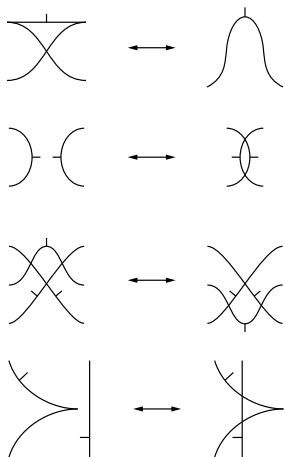
Figure 2. Moves for wavefronts on an oriented surface, with one possible choice of coorientation on each branch.
