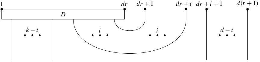
Figure 3. From diagram D to diagram D' .
