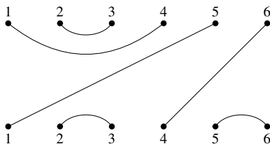
Figure 1. A planar diagram from 6 to 6.
