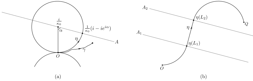
Figure 3. An illustration of (3.5) and (3.6).
