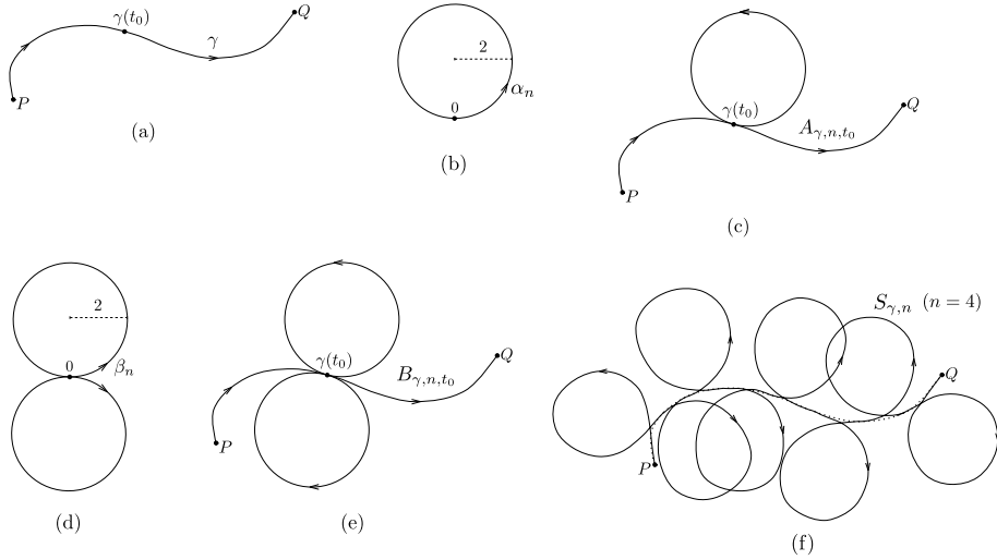
Figure 7. A depiction of how to attach loops and eights to a curve and how to spread eights along it.
