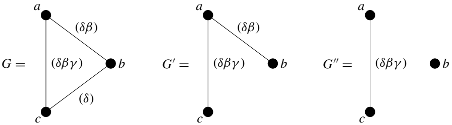
Figure 2. Graphs of Example 2.13.
