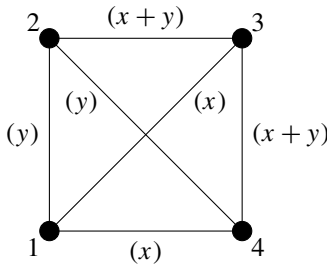
Figure 4. Graph of Example 3.8.
