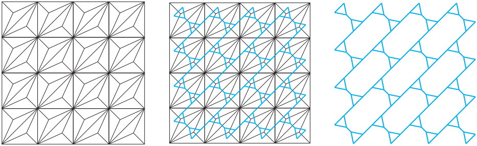
Figure 6. Dual graph for a triangulated rectangular grid.
