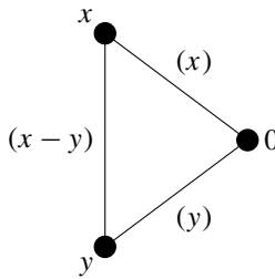
Figure 3. Graph of Example 3.7.
