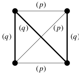
Figure 5. Graph (K_4, \alpha) of Example 3.11.
