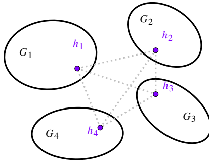
Figure 1. A generalized bridge.
