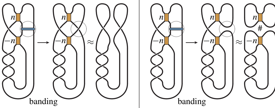
Figure 4. Left: A banding of B(3n^2 + n + 1, -3n + 2) along the arc \tau_n^* produces the unknot. Right: A different banding of B(3n^2 + n + 1, -3n + 2) along the arc \tau_n^* produces the connected sum of B(n, -1) and B(3n + 1, 3) .
