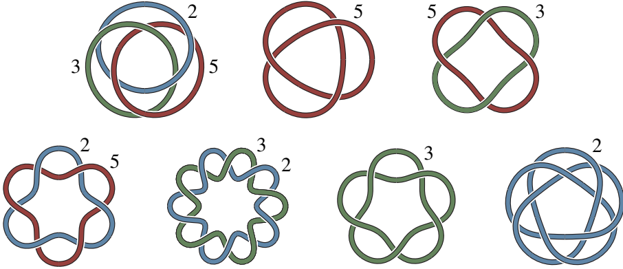
Figure 7. The possible singular sets of orbifolds cyclically covered by \mathcal{P} with underlying space S^3 . These are the relevant cases from a more general classification in [Dunbar 1988]. Following the notation of that paper, a link component labeled by n indicates a cone angle of 2\pi/n along that component in the singular set of the corresponding orbifold.
