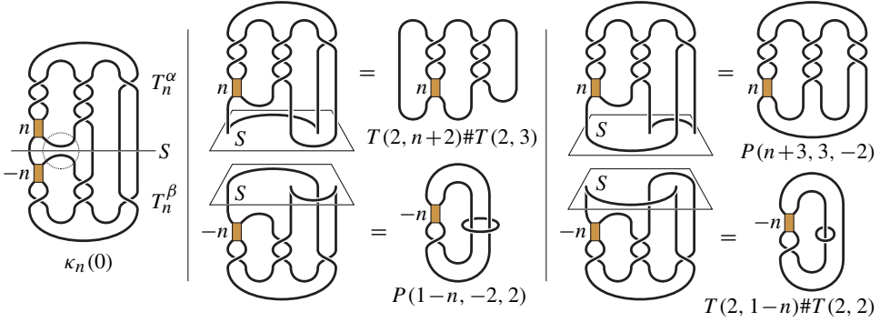
Figure 2. Left: The bridge sphere S for P(-2, 3, 5) splits \kappa_n(0) into two tangles, T_n^\alpha above and T_n^\beta below. Middle: Filling T_n^\alpha with a rational tangle to get T(2, n+2) \# T(2, 3) makes T_n^\beta into P(1-n, -2, 2) . Right: Filling T_n^\beta with a rational tangle to get T(2, 1-n) \# T(2, 2) makes T_n^\alpha into P(n+3, 3, -2) .
