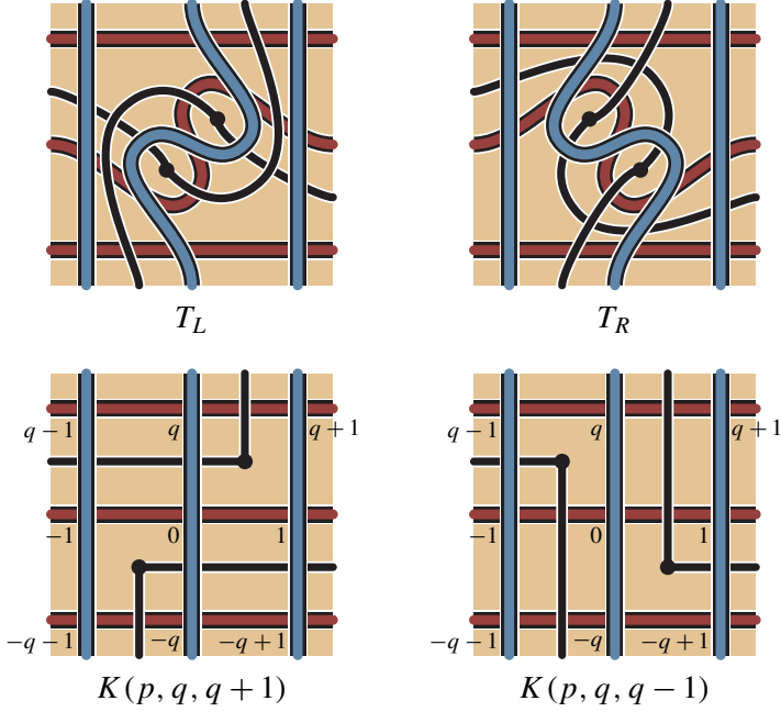
Figure 6. Local portions of the doubly pointed diagrams for the almost-simple knots T_L and T_R and their associated simple knots K(p, q, q+1) and K(p, q, q-1) ; see [Baker 2014b, Figure 1; Hedden 2011, Figure 3]. In the bottom two pictures, the intersection points of the red \alpha -curve and blue \beta -curve are numbered in order mod p along the \alpha -curve.
