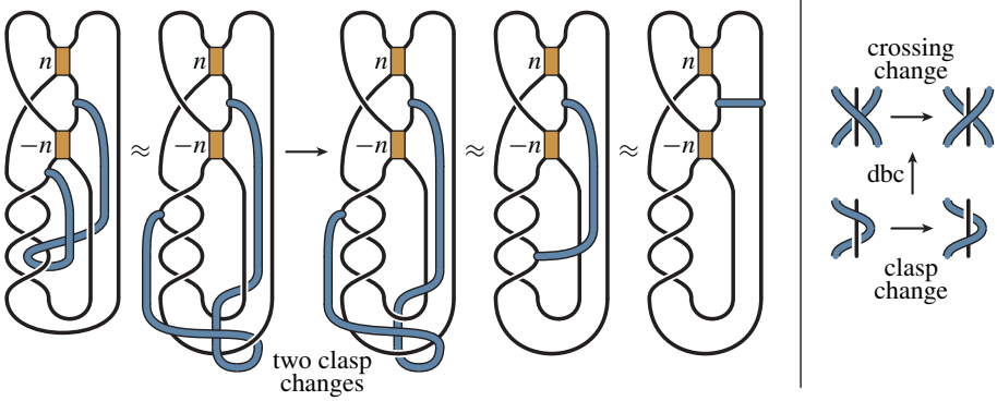
Figure 3. Left: An isotopy of the arc \kappa_n^* on the two bridge link B(3n^2 + n + 1, -3n + 2) from the lower left of Figure 1 has two clasp changes performed. The resulting arc \tau_n^* is then isotoped to lie in a bridge sphere. Right: A clasp change of an arc around a segment of a branch locus lifts to a crossing change about a segment of the fixed set in the double branched cover.
