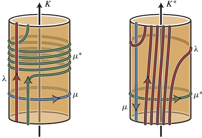
Figure 5. Left: A regular neighborhood of an oriented knot K in a homology sphere Y has meridian \mu linking K positively and longitude \lambda oriented as the boundary of a Seifert surface. The surgery curve \mu^* of positive slope 5/1 shown here is oriented as [\mu^*] = [\lambda] + 5[\mu] in H_1(\partial\mathcal{N}(K)) . Right: Performing \mu^* -surgery on K produces the rational homology sphere Z and surgery dual knot K^* . Orienting K^* to be linked positively by its meridian \mu^* , the boundary of the (rational) Seifert surface \lambda is homologous to 5[K^*] in \mathcal{N}(K^*) while the longitude \mu is homologous to -[K^*] .
