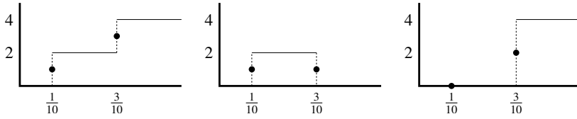
Figure 1. Signature functions for -5_1 , 10_{132} and -5_1 \# -10_{132} .
