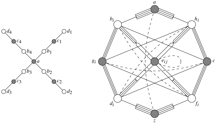
Figure 1. The X_{3333} diagram is on the left. A shorthand drawing of the 32 node diagram D is on the right. In the 32 node diagram, 1 \leq i < j \leq 4 , so the node c_i (resp. e_{ij} ) stands for four (resp. six) nodes. A solid (resp. dashed) edge between two vertices x and y indicates the relation xyx = yxy (resp. xyxy = yxyx ). No edge between x and y means xy = yx . The following shorthands are used: The edge between a and b_i means that a and b_i are connected for all i . A single (resp. triple) edge between b_i and c_i (resp. g_i ) means that b_i and c_j (resp. g_j ) are connected if i = j (resp. i \neq j ). Notice that there are two kinds of edges out of e_{ij} . The edge between e_{ij} and d_i (resp. b_i ) means that e_{ij} is connected to d_k (resp. b_k ) if k \in \{i, j\} (resp. k \notin \{i, j\} ). Finally, the dashed loop joining e_{ij} to itself means that e_{ij} is joined to e_{kl} by a dashed edge if \{i, j\} \cap \{k, l\} = \emptyset .
