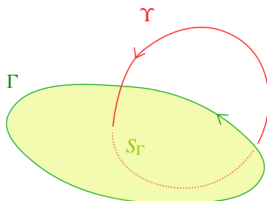
Figure 1. Here, both collections \Gamma and \Upsilon consist of a single curve. Their linking number is \pm 1 , depending on the global orientation.
