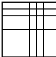
Figure 5. A grid pattern.
