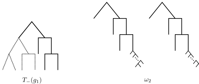
Figure 9. An example of the construction of \omega_2 . The dotted carets in T_-(g_1) are not used when constructing \omega_2 . The all-right tree T'_-(g_1) is obtained by removing the dotted carets from T_-(g_1) . Note that the tree T'_-(g_1) is the domain tree of the product C_{m_1} \cdots C_{m_p} . By using T'_-(g_1) , all we needed to define \omega_2 are the generators \hat{B}_0 , x_0 , and x_1 . See also Figure 10.
