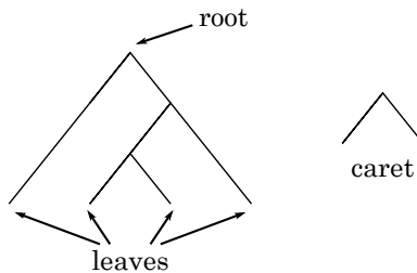
Figure 2. A binary tree and a caret.
