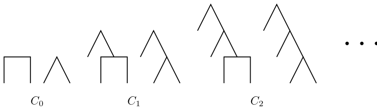
Figure 7. Generators C_0, C_1, \dots
