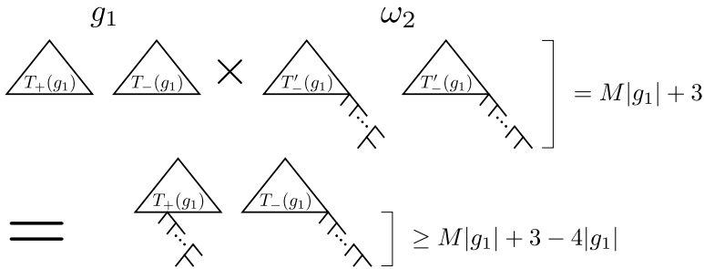
Figure 10. An illustration of the multiplication of g_1 and \omega_2 , where (T_+(g_1), T_-(g_1)) is a minimal pair of colored binary trees of g_1 and T'_-(g_1) is the maximal all-right colored binary tree contained in T_-(g_1) .
