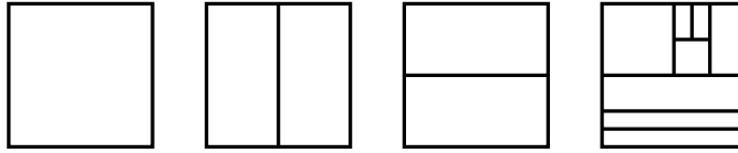
Figure 1. The trivial pattern, the pattern once divided vertically, the pattern once divided horizontally, and a pattern.
