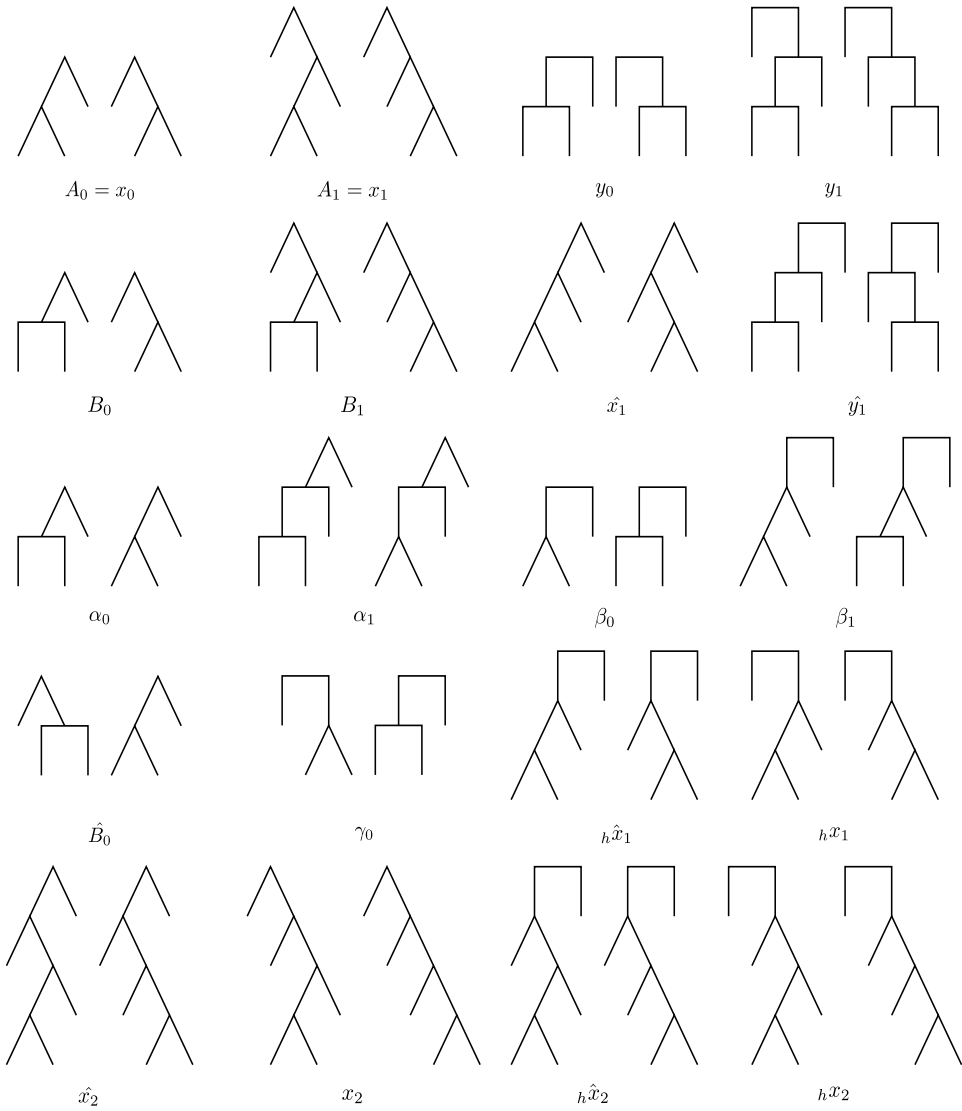
Figure 6. Generators of 2V except C_0, C_1, \pi_0, \pi_1, \overline{\pi_0} , and \overline{\pi_1} .
