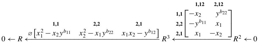
Figure 2. The Apéry resolution for m = 3 .
