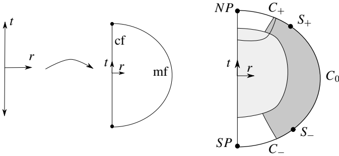
Figure 1. The compactification M of \mathbb{R}_t \times (0, \infty)_r \times Z with the Z factor suppressed, mapping on the left with detail on the right. The image of \mathbb{R}_t \times (0, \infty)_r can be thought of either as the right half disk D_+ or the quarter-sphere \mathbb{S}_{++} . S_{\pm} are, respectively, collapsed future/past null infinity. C_{\pm} and C_0 are three subsets of mf corresponding to past and future timelike infinity and spacelike infinity, respectively.
