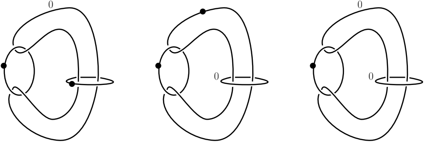
Figure 2. A trick due to Moishezon [30] as explained by Gompf in [19, proof of Lemma 3].
