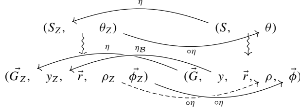
Figure 4. Relationship between the corresponding J.-K. Yu data given the relationship between the tame F -nonsingular elliptic pairs.
