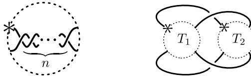
Figure 2. Left: The tangle Q_n . Right: The link \mathcal{L}(T_1, T_2) .
