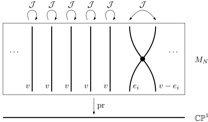
Figure 1. Each line represents a copy of \mathbb{CP}^1 and is labeled with its homology class in M_N . The rightmost fiber, for 1 \leq i \leq N - 1 , is a singular fiber. Each singular fiber is a union of two (-1) -spheres intersecting transversely once.
