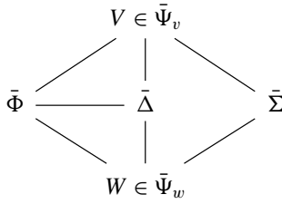
Figure 3. The simplices involved in the construction of Lemma 5.11, where edges denote joins in \bar{X} . Actually, \bar{\Sigma} and \bar{\Delta} \star \bar{\Phi} need not be disjoint, but none of them can contain V or W .
