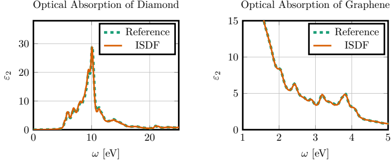
Figure 4. Optical absorption spectrum for diamond (left) and graphene (right).
