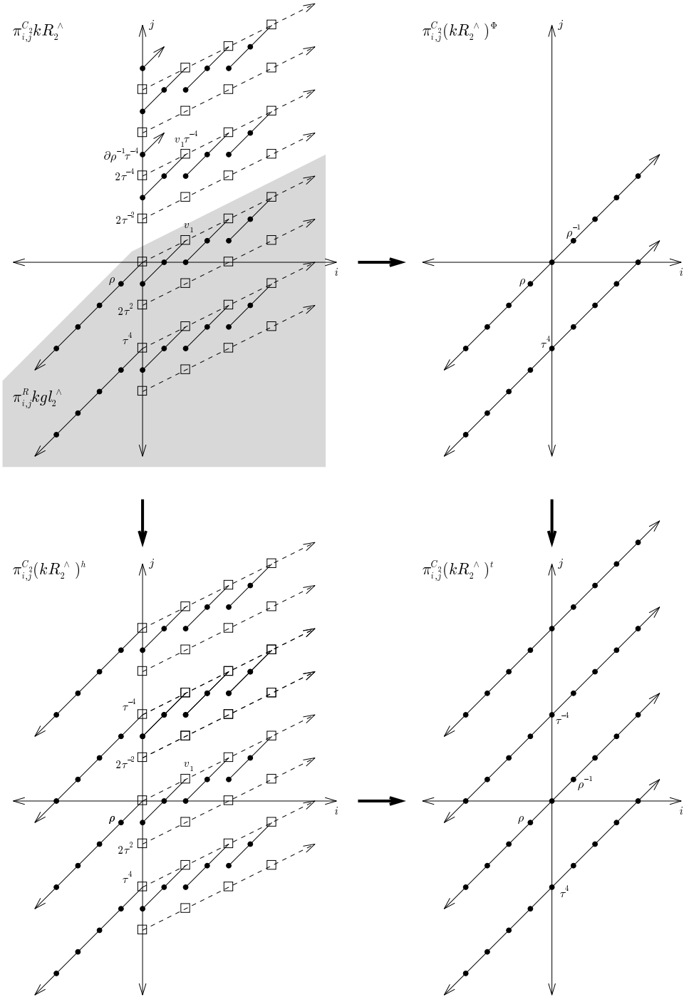
Figure 4. Computing \pi_{*,*}^{C_2} kR_2^{\wedge} from \pi_{*,*}^{\mathbb{R}} (kg l_2^{\wedge})_{\mathbb{R}} .
