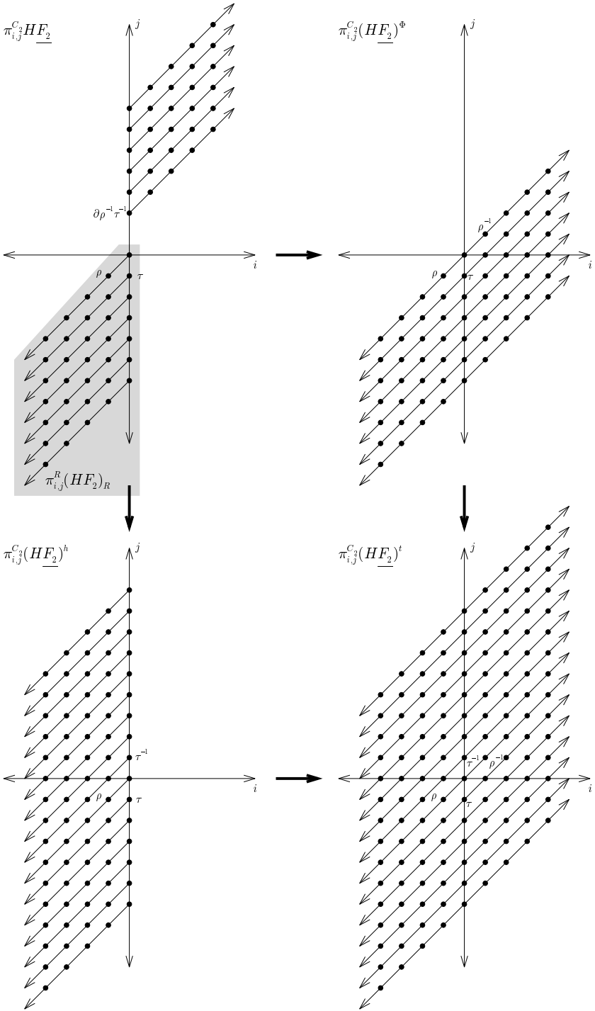
Figure 2. Computing \pi_{*,*}^{C_2} \underline{HF}_2 from \pi_{*,*}^R(\underline{HF}_2)_R .
