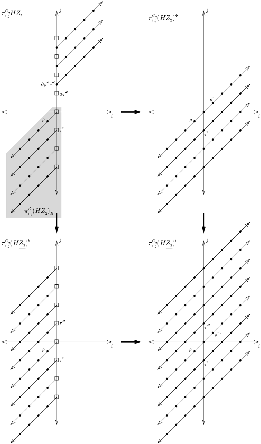
Figure 3. Computing \pi_{*,*}^{C_2} H\underline{\mathbb{Z}}_2 from \pi_{*,*}^{\mathbb{R}}(H\underline{\mathbb{Z}}_2)_{\mathbb{R}} .
