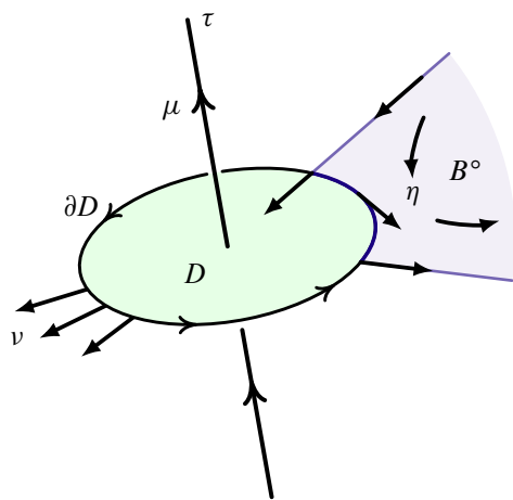
Figure 9: How \eta twists with respect to v near a mixed edge \tau .
