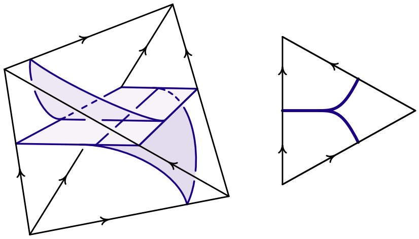
Figure 6: The branched surface B(\mu) in one tetrahedron. Note that each face of the tetrahedron looks like the figure at right, and hence these local pictures glue up to give a branched surface in \mathcal{T} .
