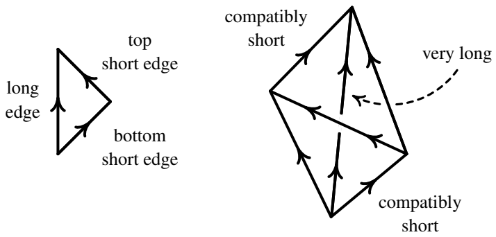
Figure 5: Local possibilities for acyclic edge orientations.
