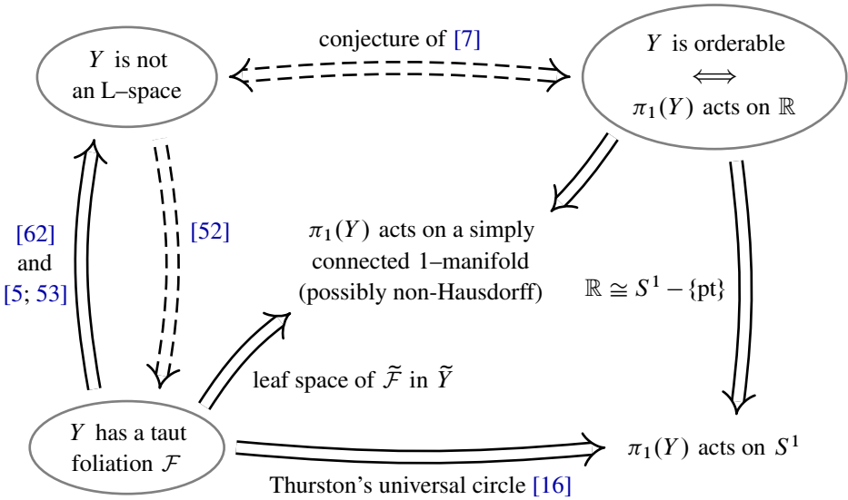
Figure 1: Some results related to Conjecture 1.2, which asserts the equivalence of the three circled conditions. Here Y is an irreducible \mathbb{Q} –homology 3–sphere, all foliations are coorientable, and all actions are nontrivial, faithful, and orientation-preserving; the solid arrows are theorems and dotted ones conjectures. See [7] for a complete discussion. This figure is copied from [19].
