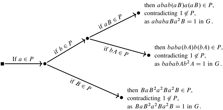
Figure 4: This figure illustrates the proof of Theorem 9.1 of [16], namely that the group G = \langle a, b \mid ababaBa^2B, ababAb^2Ab \rangle is not left-orderable; here A = a^{-1} and B = b^{-1} . (The group G is the fundamental group of the Weeks manifold.) The nonordering tree should be read starting from the leftmost vertex and encodes a proof by contradiction: we assume that a positive cone P exists, and then consider all possibilities for whether certain nontrivial elements of G are or are not in P . In each case, the contradiction comes from showing that P \cdot P \subset P implies that 1 \in P . Because we can reverse the roles of P and P^{-1} , we need not consider the case when A \in P .
