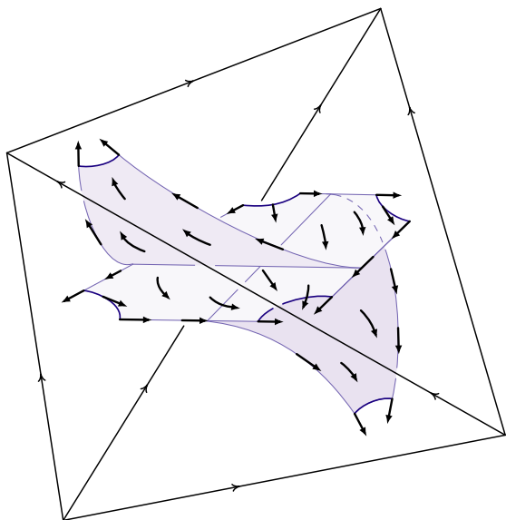
Figure 8: The section \eta of UTB^\circ in each tetrahedron of \mathcal{T} .
