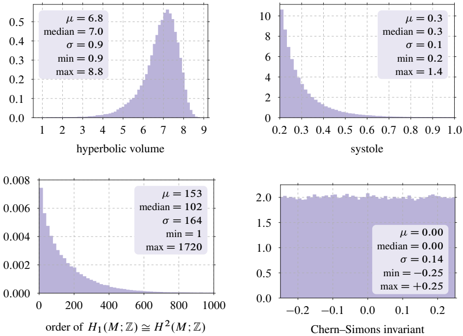
Figure 3: Some basic geometric and topological statistics about the manifolds in \mathcal{Y} given as histograms. For similar plots about \mathcal{C} , see [23].
