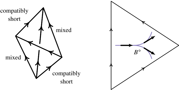
Figure 7: The mixed edges of an acyclically oriented tetrahedron (left) and the section \eta of UTB^\circ in each face of \mathcal{T} (right).
