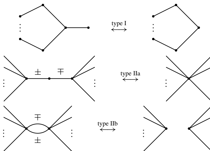
Figure 5: The Reidemeister moves relevant to this paper. A move of type I allows us to add (or remove) a 1-valent vertex and its edge. In the presence of a 2-valent vertex whose edges have opposite signs, the two edges may be contracted according to a move of type IIa. In a move of type IIb a pair of parallel edges with opposite signs may be added (or removed).
