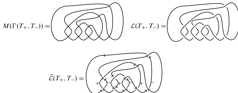
Figure 3: From the medial graph of a \Gamma -graph to an oriented link.
