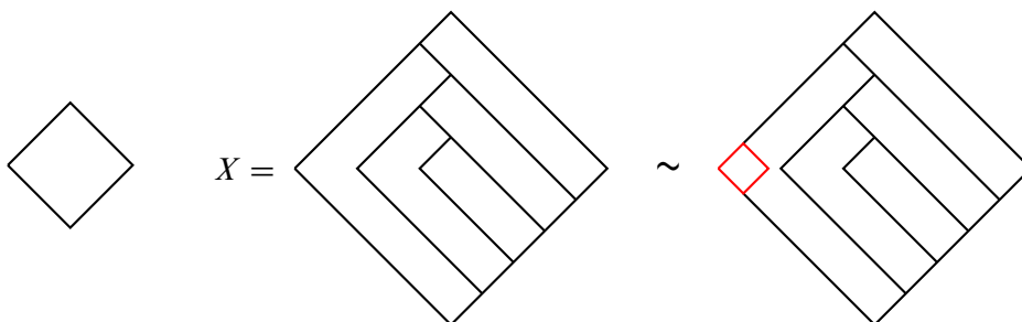
Figure 1: A pair of opposing carets and two equivalent elements in F .
