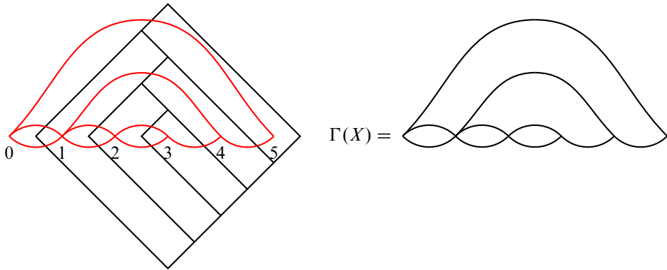
Figure 2: An example of a \Gamma -graph.
