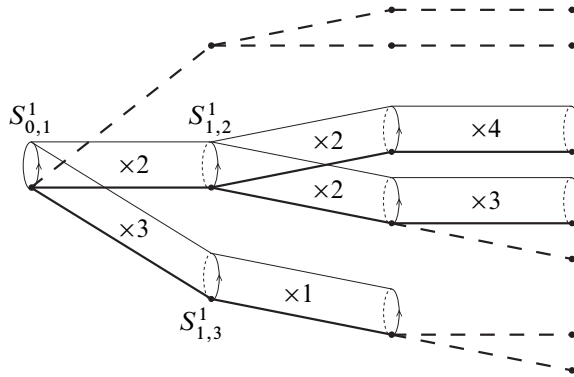
Figure 2: Model base space X_\Gamma corresponding to Figure 1.
